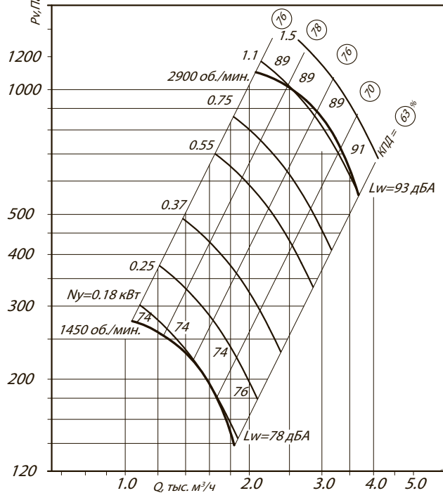
D=0.95D
