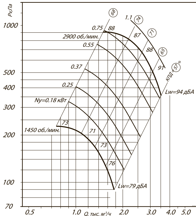
D=0.9D
